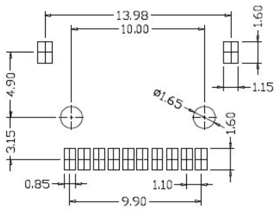
RECOMMENDED PCB LAYOUT ТПР VTFW (.XX±0.05)
