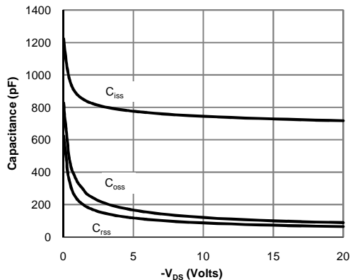
Figure 8: Capacitance Characteristics
