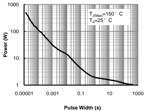
Figure 10: Single Pulse Power Rating Junction-to-Ambient (Note F)
