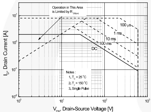
Figure 9-1. Maximum Safe Operating Area for FQP2N60C
