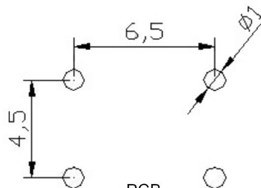
PCB
