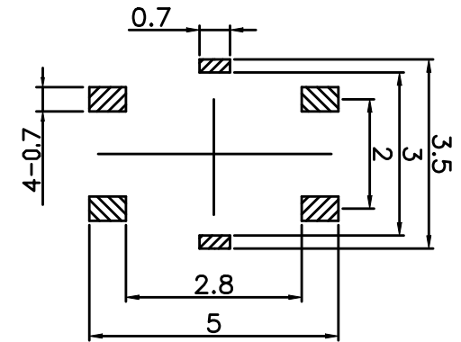
Schematic PCB
