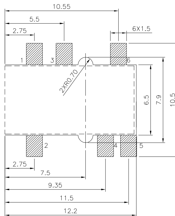
Recommended P.C.B. Layout(Top View)
